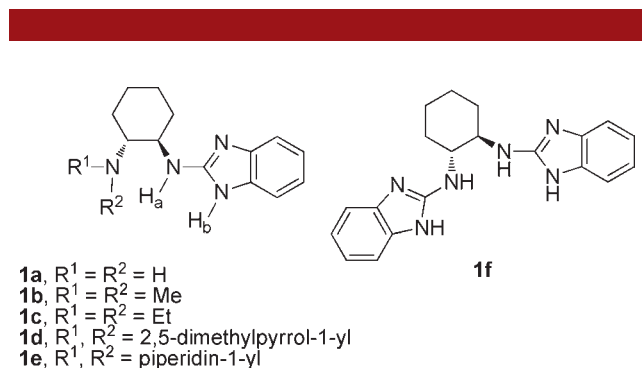
Figure 1. Hydrogen bond donor catalysts.
