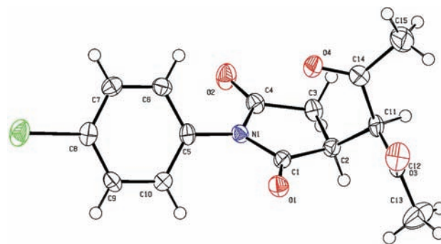
Figure 2. X-ray structure for compound 2e .
